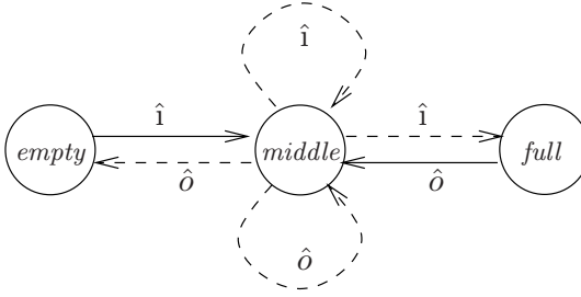
Fig. 7.2. The abstracted state space of a bag of size N
