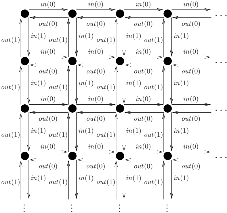
Fig. 3.2. State space of the bag over \{0, 1\}
